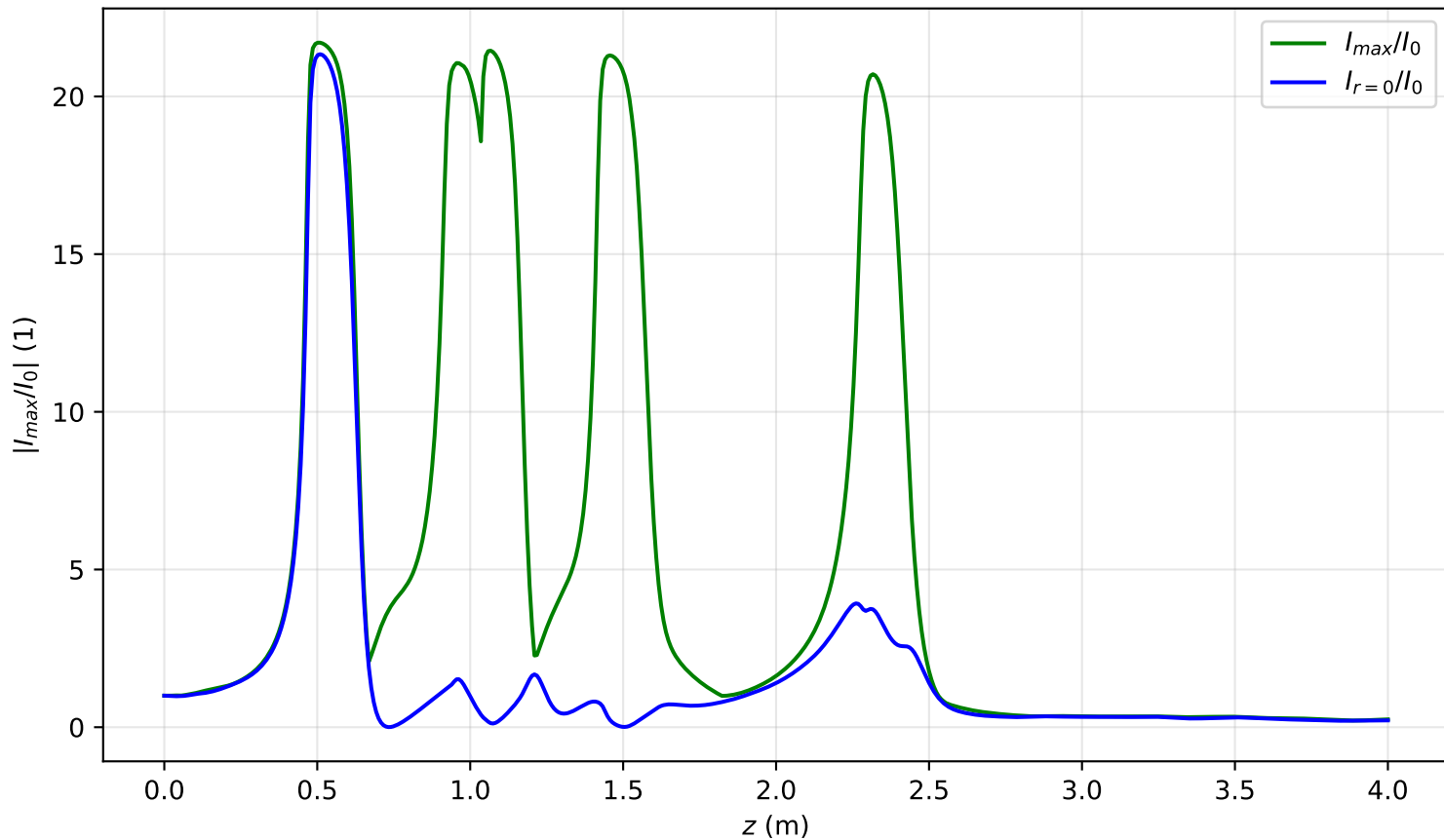
I_{max}(x=0, y=0, z)/I_0 , Pin=5.1Pcr, noisy input, artificial time
